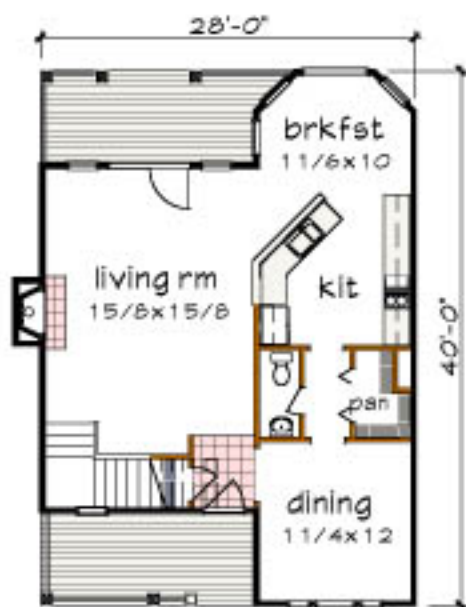
Floor 1 plan
